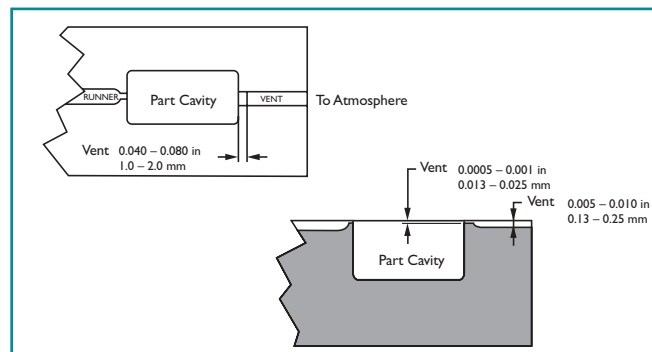
Figure 6. Example of appropriate venting.
