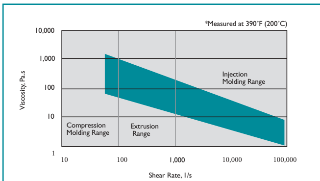
Figure 15. The effect of shear rate on the viscosity of GLS styrenic TPEs.
